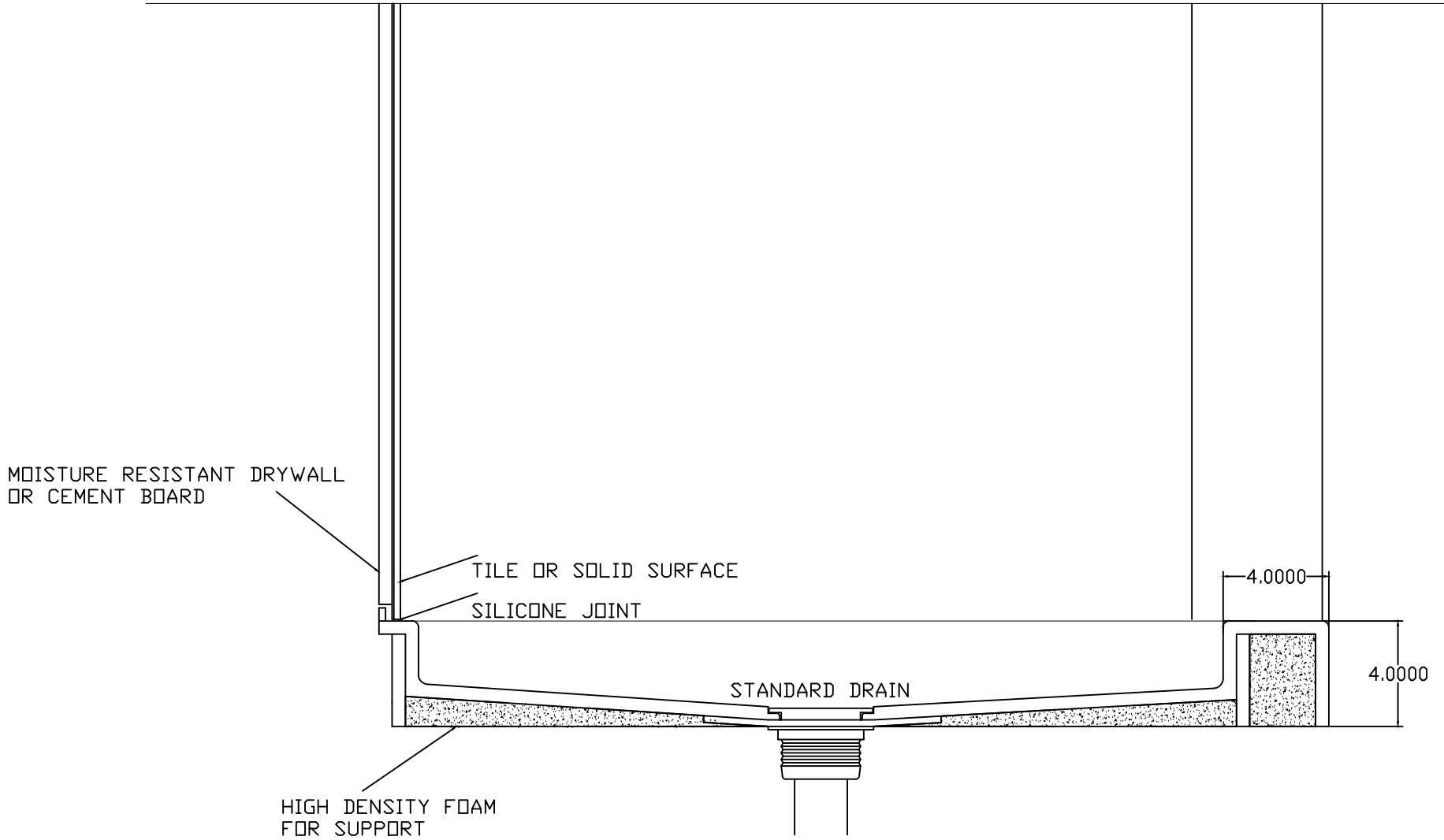
SIDE VIEW STANDARD HEIGHT THRESHOLD
