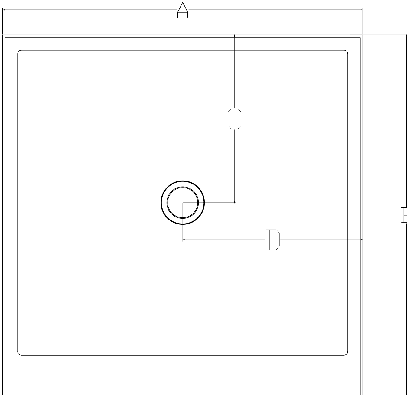
PLAN VIEW STANDARD HEIGHT THRESHOLD
