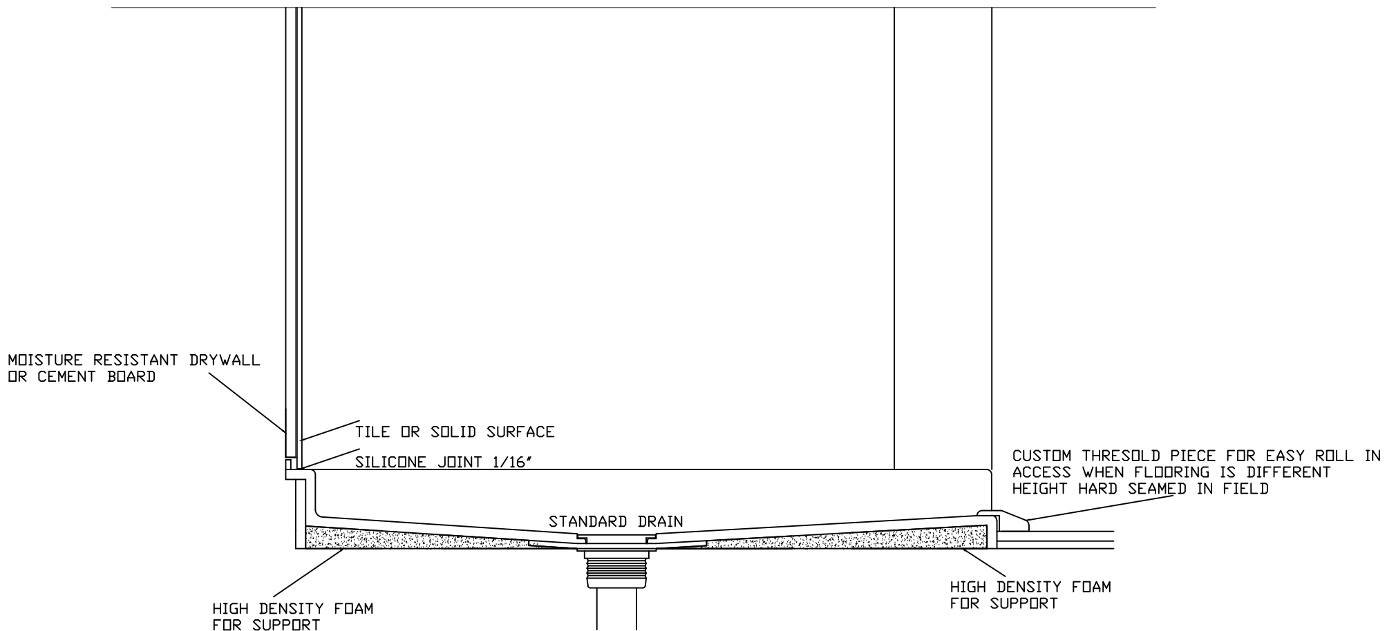
SIDEVIEW ADA NO CURB SHOWER PAN WITH APPLIED THRESHOLD TO MEET FLOORING DIFFERENCES
