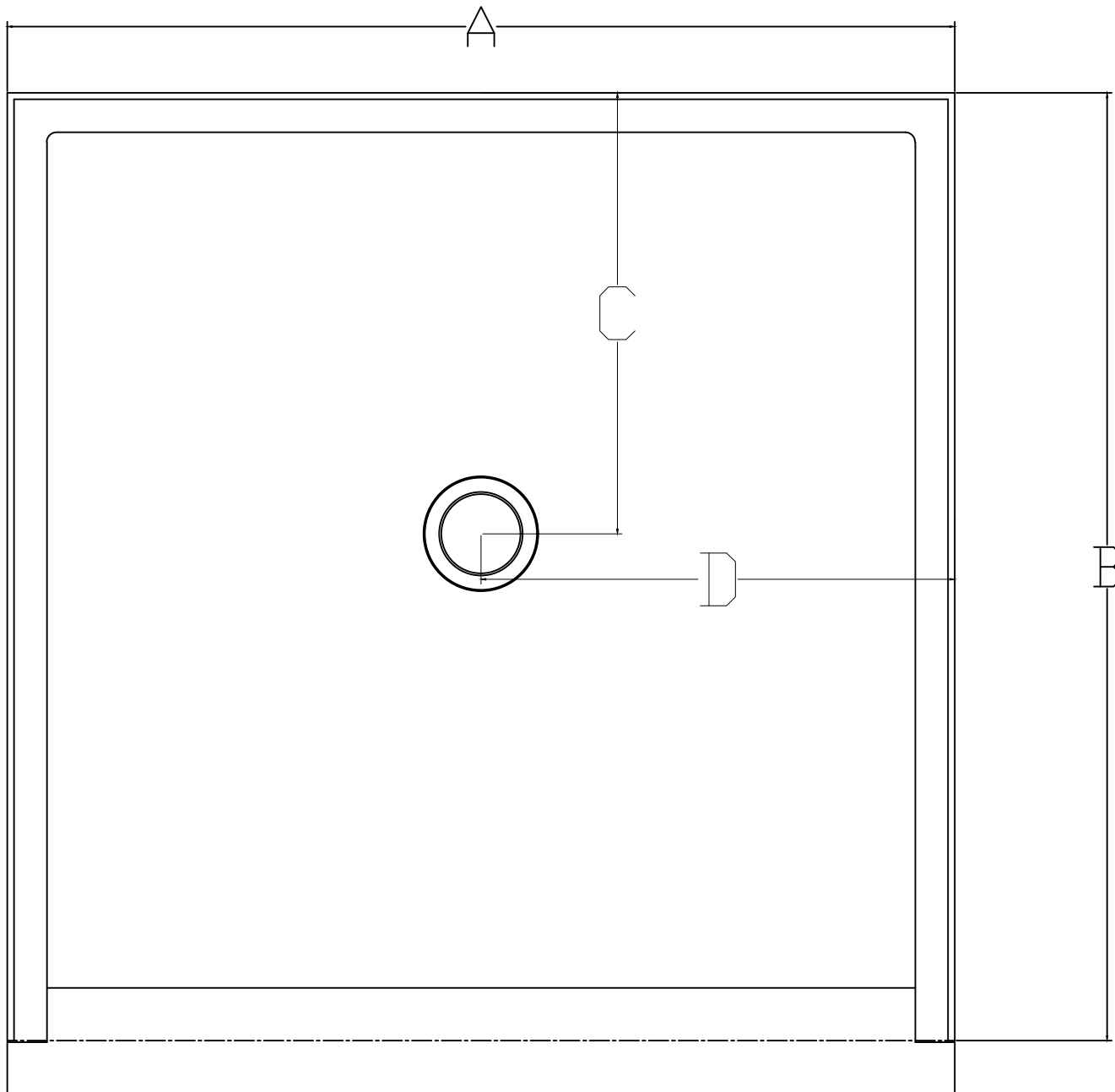
PLAN VIEW ADA NO CURB SHOWER PAN WITH APPLIED THRESHOLD TO MEET FLOORING DIFFERENCES
