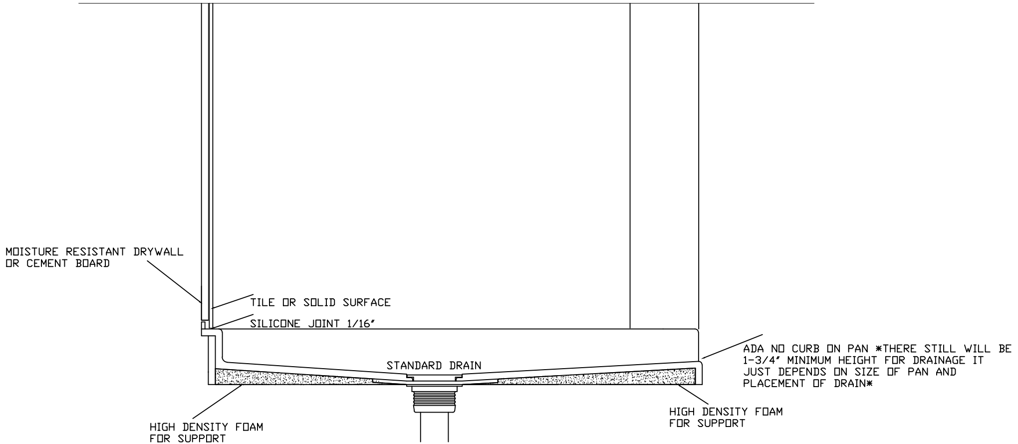
SIDE VIEW ADA NO CURB SHOWER PAN
