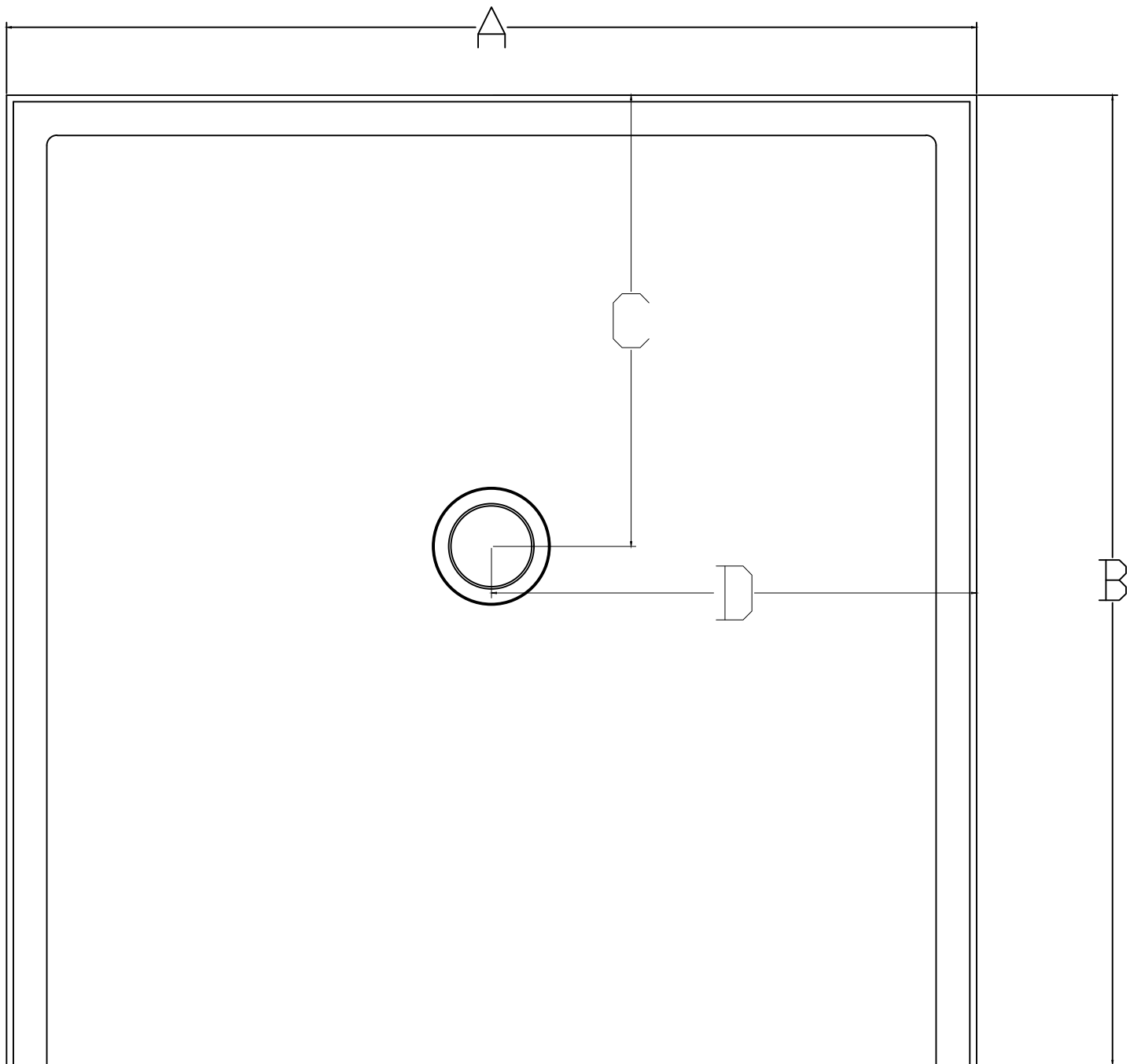
PLAN VIEW ADA NO CURB SHOWER PAN
